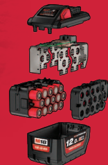
REDLITHIUM™-ION BATTERY PACK
